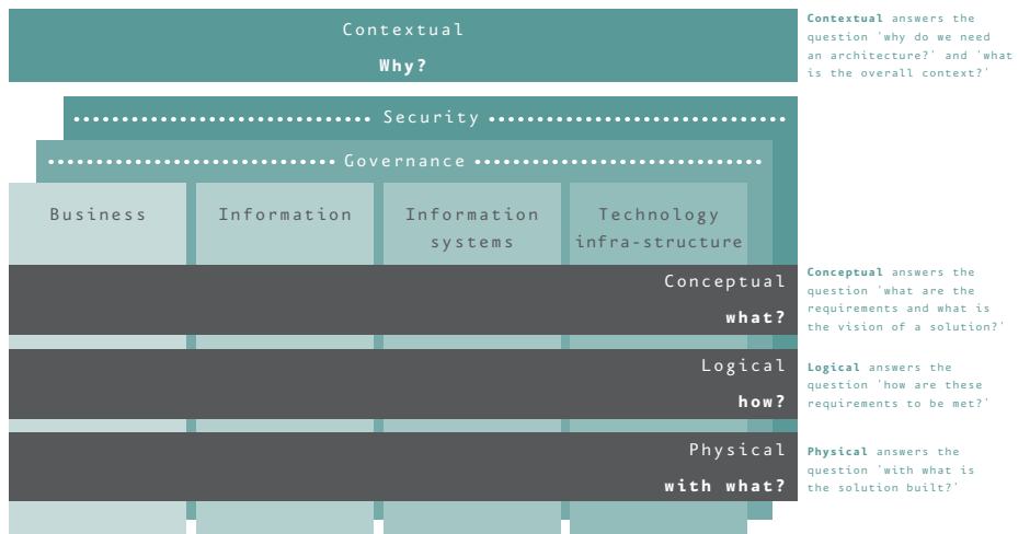
Figure 2. Integrated Architecture Framework
