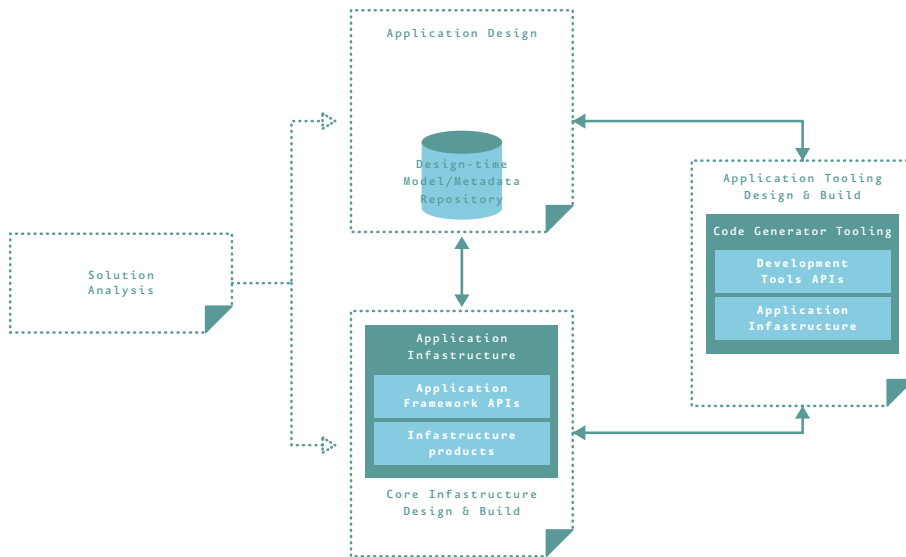
Figure 4. A metadata-driven process
