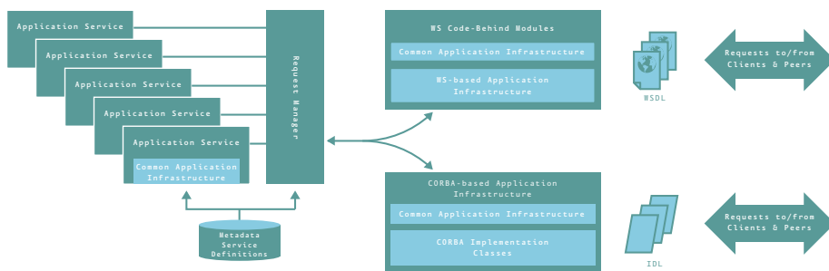
Figure 6. Request processing
