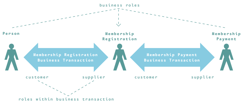
Figure 7. Business roles
