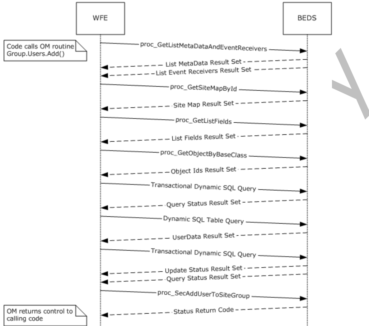
Figure 3: Group Add User To Site Group OM
