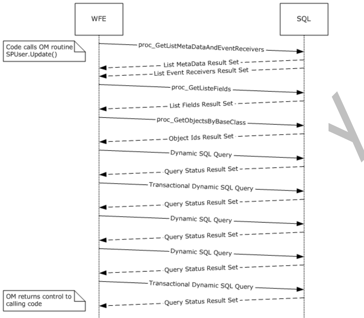
Figure 17: User Update User Properties OM
