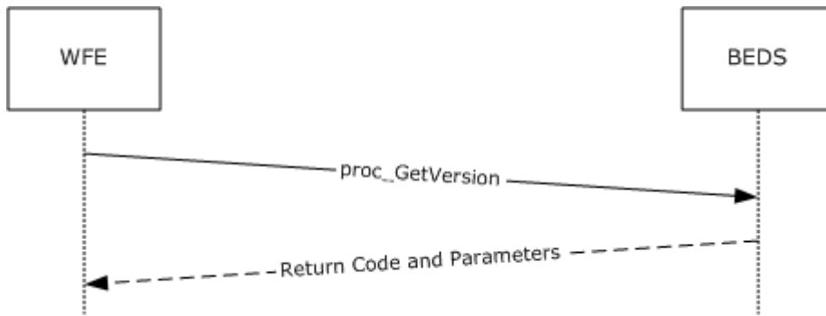
Figure 18: Version Negotiation
