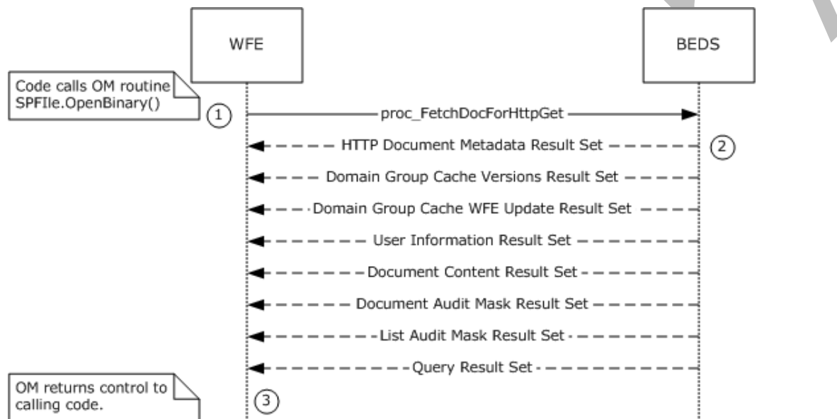
Figure 2: File: Open File OM
