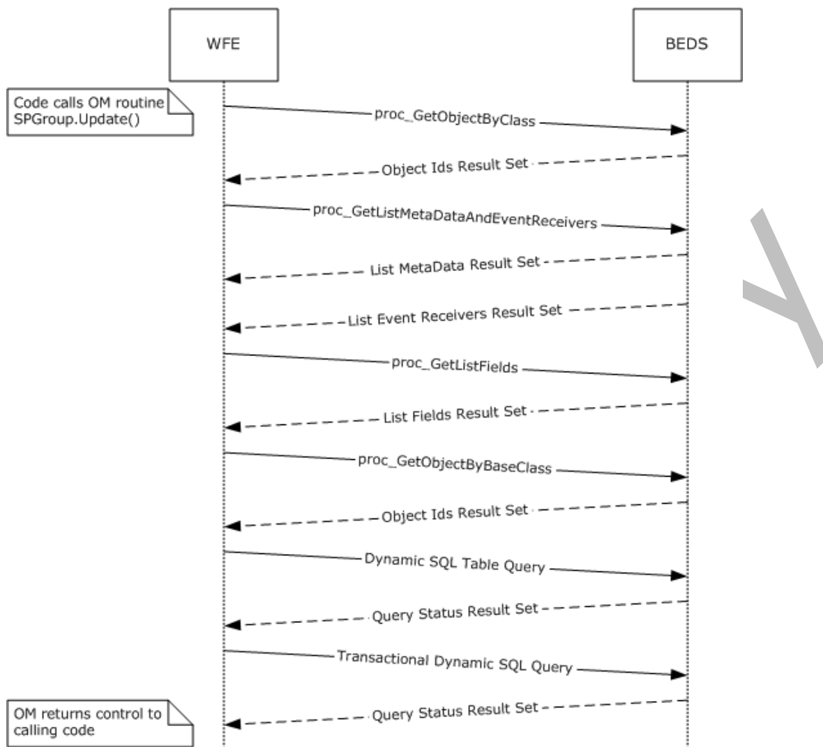
Figure 4: Group Update Site Group Properties OM
