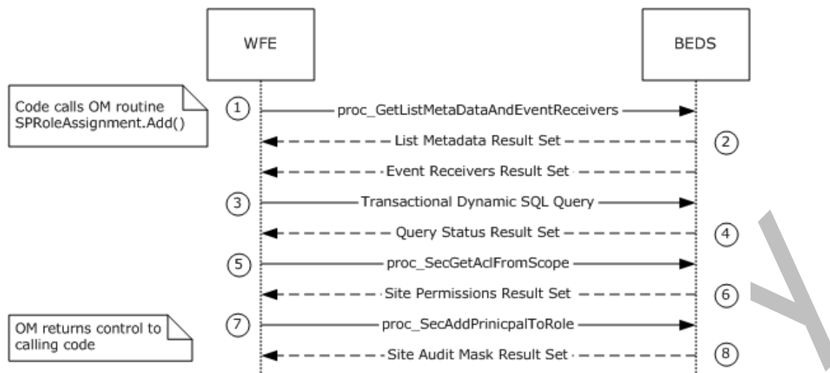
Figure 5: Add User to Document Library via Object Model
