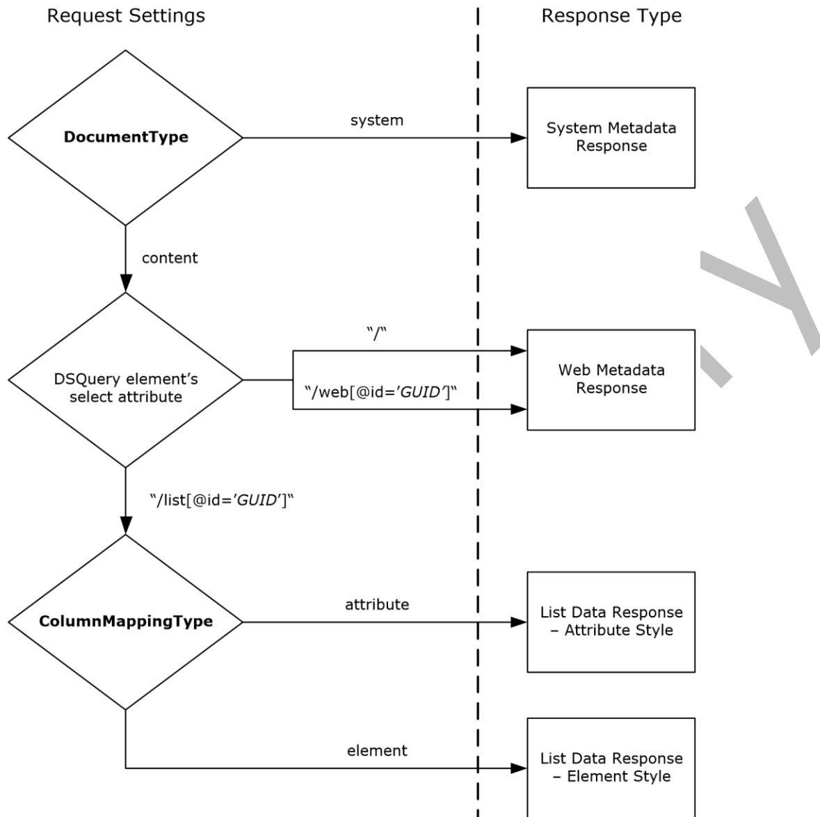
Figure 2: How various request settings determine the response type
