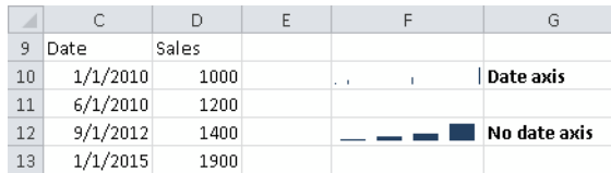
FIGURE 44-7 Sparklines with a data axis.
