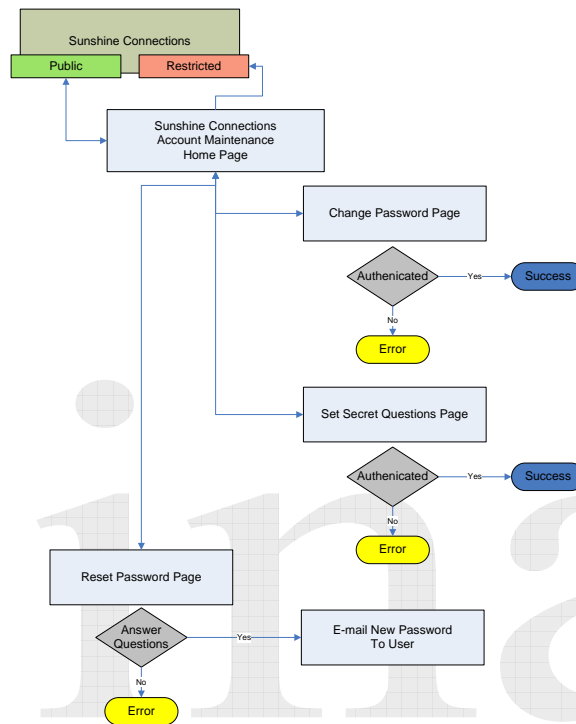
Figure 1 – Account Maintenance System Overview
