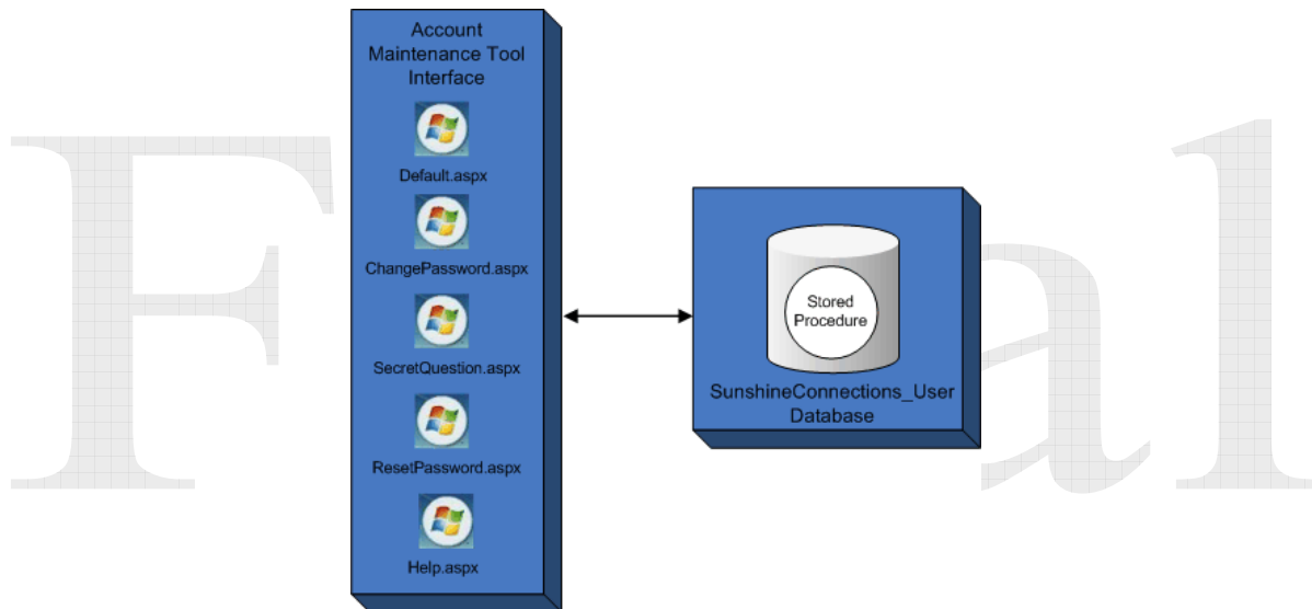
Figure 7 – Account Maintenance Deployment Diagram
