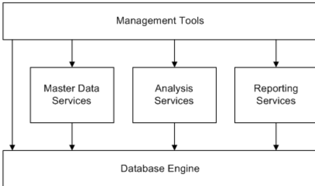
Figure 14: Using management tools to set up the system
