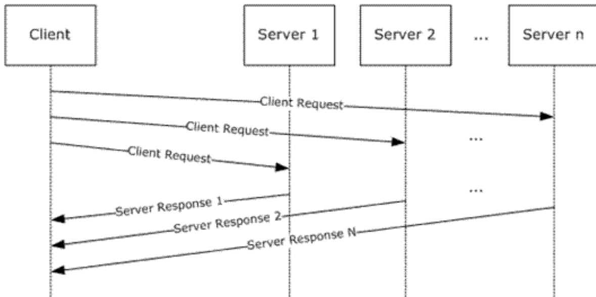
Figure 10: SQL Server instance discovery use case
