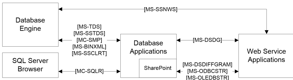
Figure 2: Network connectivity and application development architecture
