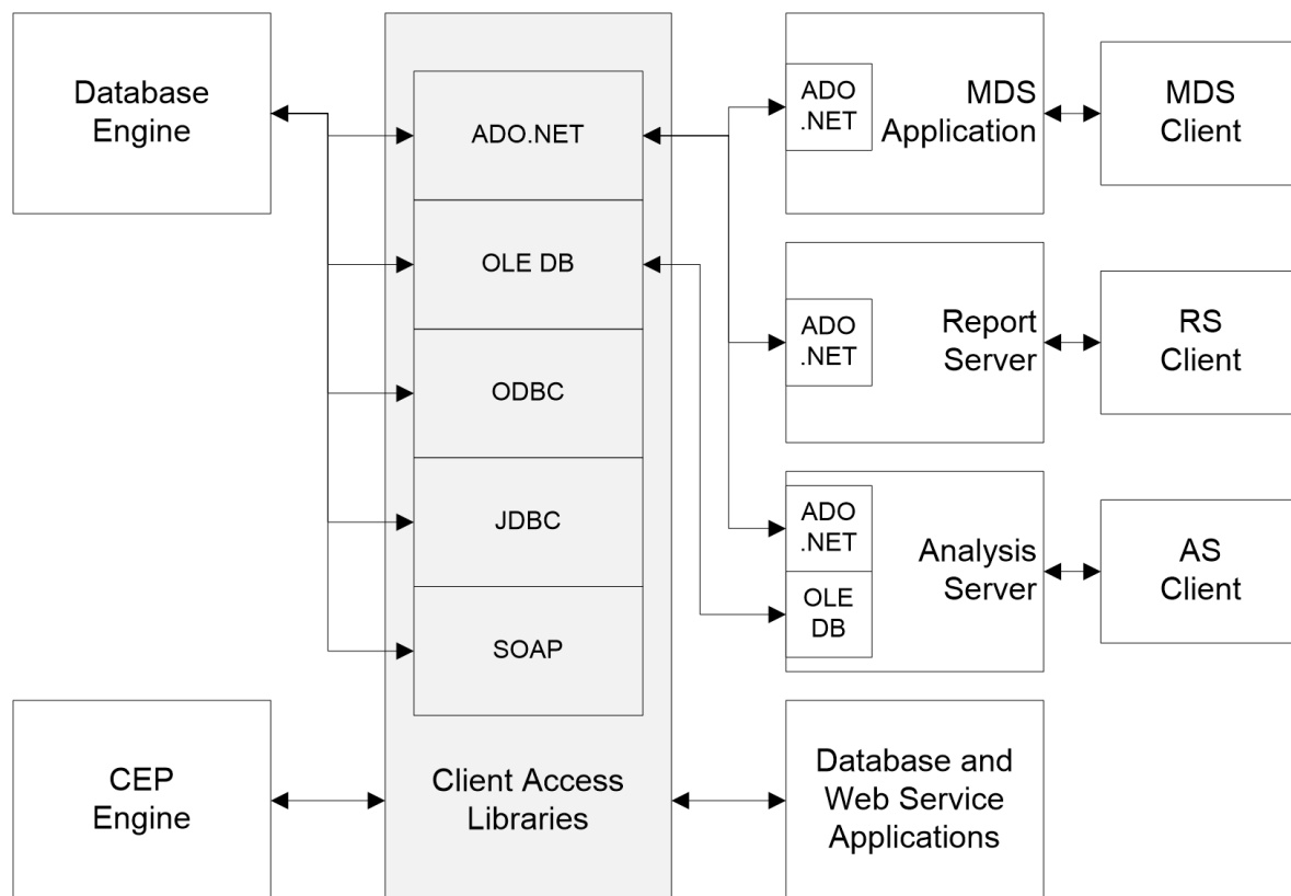
Figure 1: SQL Server architecture overview
