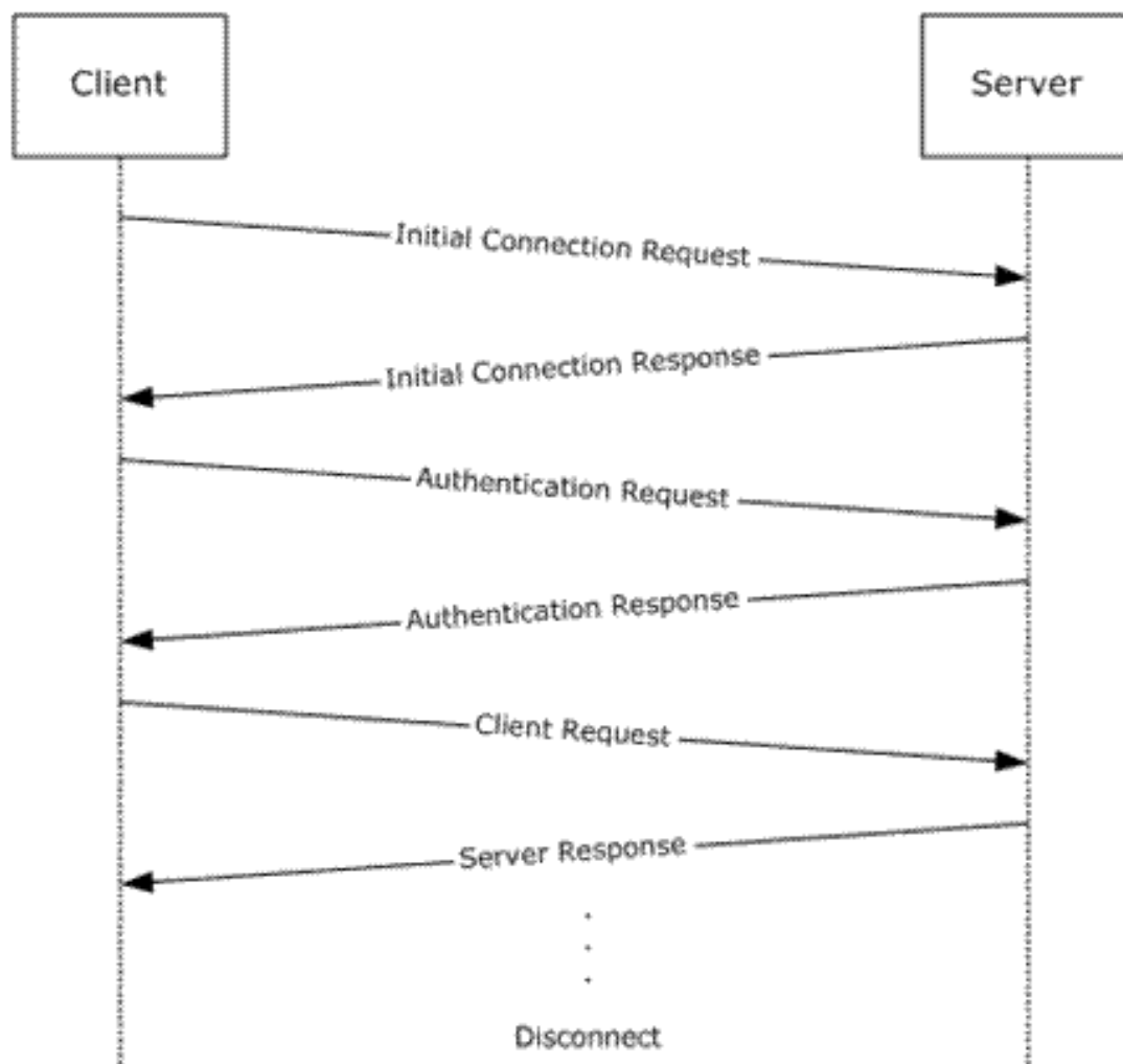
Figure 12: Client connection use case
