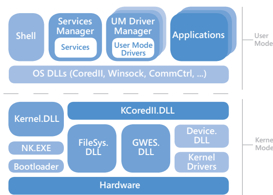
The CE 6.0 OS layout featuring the new unified kernel.
